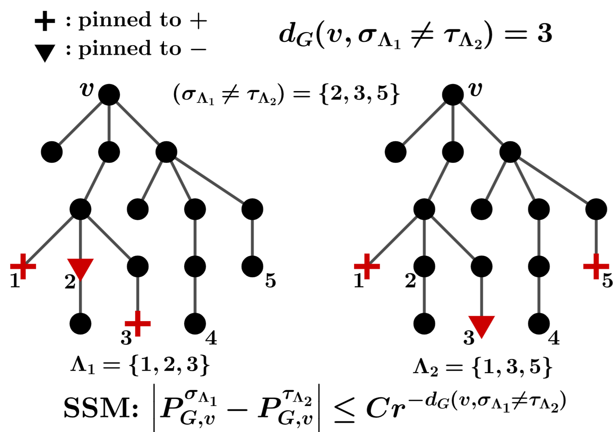
Figure 1: Strong Spatial Mixing
