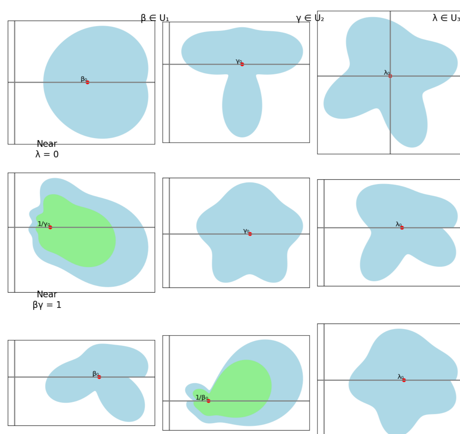
Figure 2: Regions in our result
